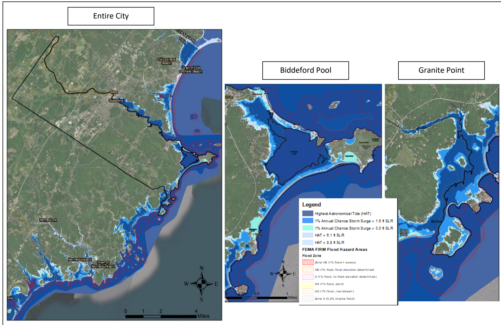
Figure 11a. Modeled inundation from sea level rise (SLR), storm surge, and the 1% annual chance storm event (Special Flood Hazard Area depicted on the FEMA-Issued Flood Insurance Rate Map).
