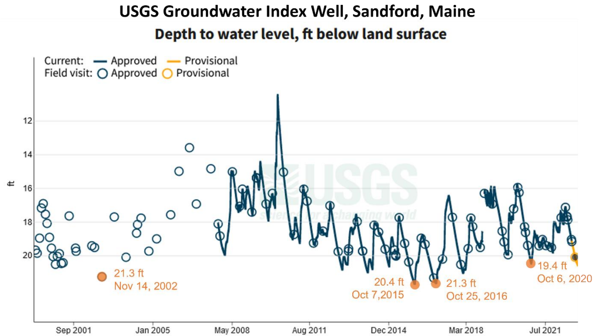
Figure 26. Groundwater levels in York County measured at an index well in Sanford, 2001-2021. Data source. United States Geological Survey
