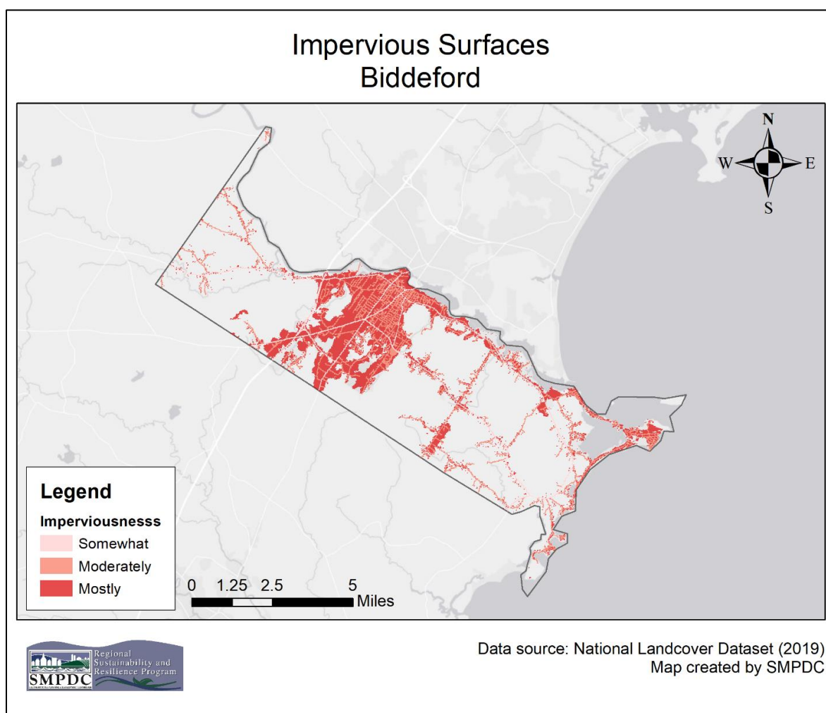
Figure 10. Impervious surfaces in Biddeford based on their level of imperviousness (somewhat, moderately or mostly impervious). Data is from the 2019 National Landcover Dataset .
