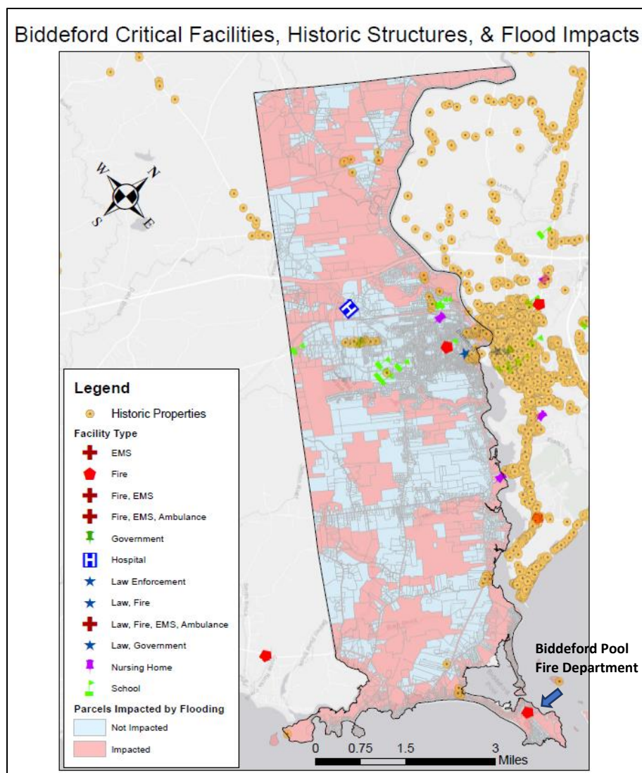
Figure 14. Mapped locations of historic properties, emergency management and public health facilities, and schools. Parcels are color-coded based on if they are projected to be directly impacted by flooding from the 1%-annual chance event (e.g., the FEMA regulatory floodplain), 1.6 feet of sea level rise, and/or 3.9 feet of sea level rise. (Source: SMPDC EDA disaster grant study, phase 2)
