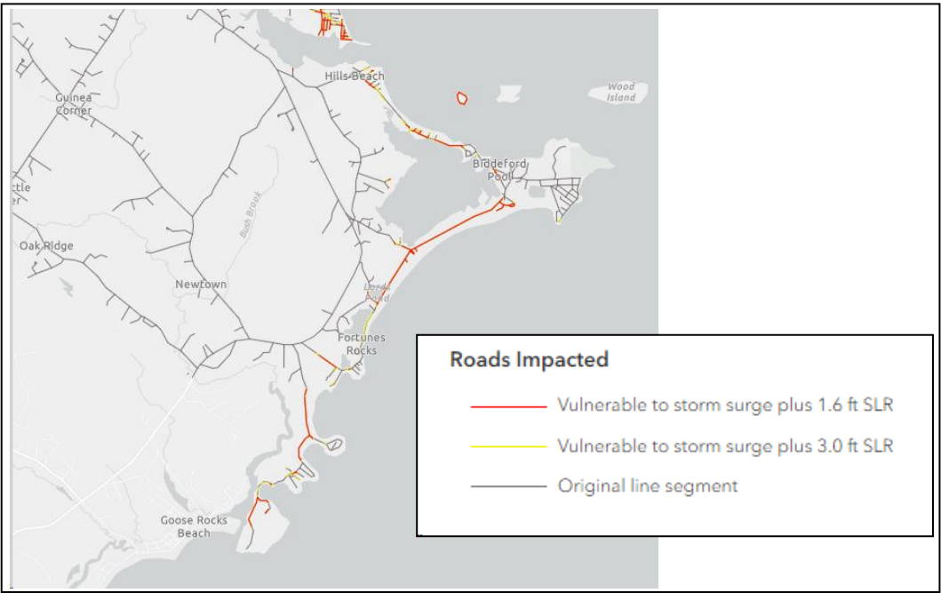
Figure 13. Roads impacted by storm surge plus sea level rise. (Source: SMPDC. 2022 coastal economic resilience assessment, phase 2. Unpublished.)
