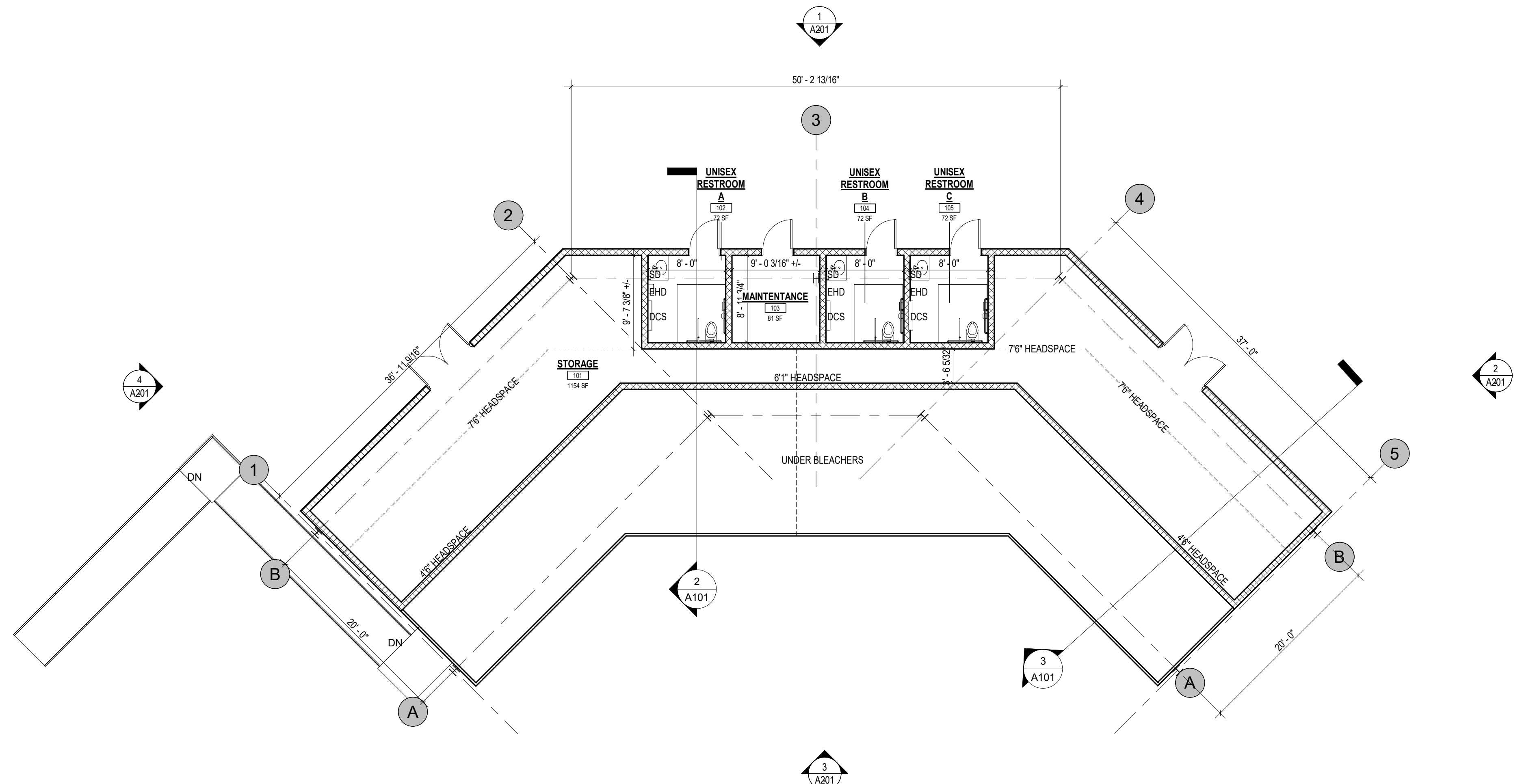
1 OVERALL FIRST FLOOR PLAN 1/8" = 1'-0" 2/ A101
